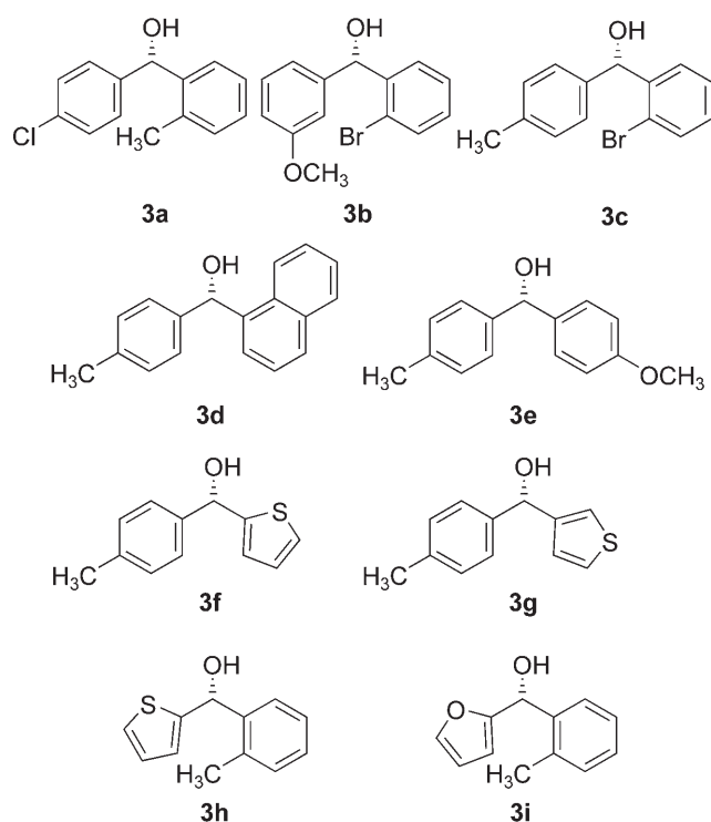
Figure 1. Products prepared by aryl transfer to aromatic aldehydes.
