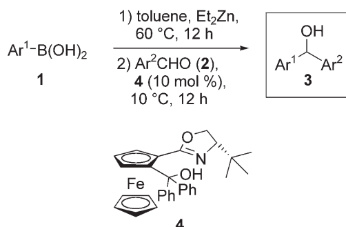
Scheme 1. Aryl transfer to aromatic aldehydes.
